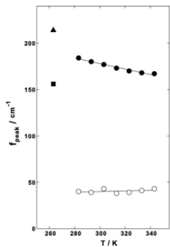
Fig. 6. Peak frequency against absolute temperature. Closed circles are peak frequencies for the S-band in water. Open circles are for the S-band in water. A closed triangle and a closed square are for two peaks of S-band in ice. Solid lines were calculation results of linear regression.
