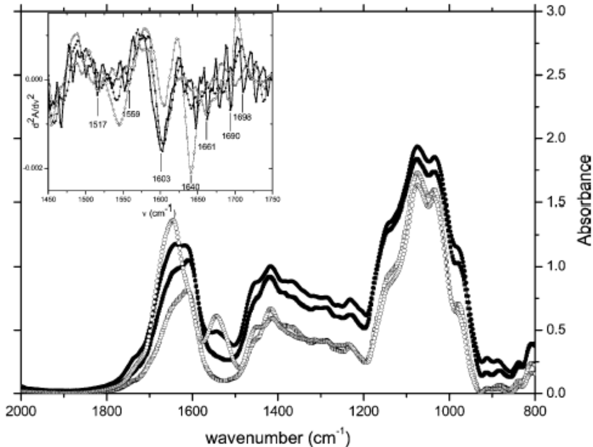
Figure 9. Infrared spectra of acacia gum, molecular fractions I, II, and III obtained after hydrophobic interaction chromatography in their solid state. (■) Total gum, (□) fraction I, (●) fraction II, and (○) fraction III. Inset: second derivative spectra associated to vibrational amide I and II bands (1750–1450 \text{cm}^{-1} )
