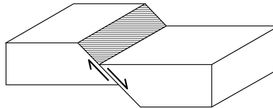
Normal dip-slip fault ( \lambda = -90^\circ )
