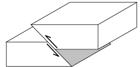
Reverse dip-slip fault ( \lambda = 90^\circ )
